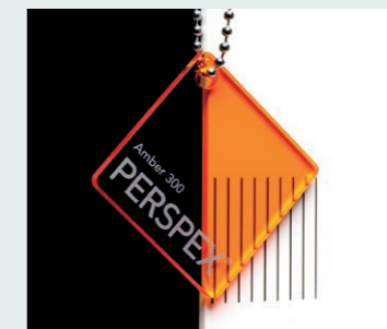
Colour: Amber Code: 300 Dimensions(mm): 3050 x 2030 Thickness (mm): 3, 5 Light Transmission (%): 38
